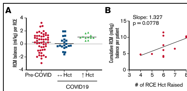
Figure 2. RCM balance in patients for whom the hematocrit was or was not consistently raised for RCE during COVID-19. (A) Average RCM balance (mL/kg) per RCE in patients pre-COVID-19 (n = 50) and for whom the hematocrit was consistently raised ( \uparrow Hct, n = 11) or not ( \leftrightarrow Hct, n = 20) during COVID-19. (B) Cumulative RCM (mL/kg) balance and number of procedures per patient in which the hematocrit was raised consistently ( \bullet represents individual patients, n = 11).
