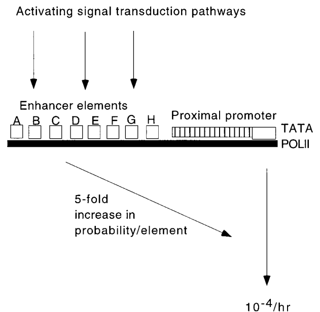
Figure 1. Probabilistic activation of a typical promoter. The diagram shows a typical inducible eukaryotic promoter. The basal promoter of the gene contains recognition sequences for abundant nuclear proteins such as Sp1, so that if the gene is in active chromatin, the elements are occupied. The minimal promoter ensures that there is a finite intrinsic low probability of recruitment of TATA-binding protein, and correct assembly an initiation complex including RNA polymerase II (POLII). The cell receives multiple independent signals simultaneously. Some of these may be autocrine, including products of the gene itself. Each signaling pathway increases the frequency with which the distal elements (A-H) are occupied. Each occupied site multiplies the probability of a pulse of transcript so that their effects in combination increase the frequency of transcription exponentially. Activation to a probability of one event per hour would be sufficient to ensure that in each cell at least one allele produces a pulse of transcript within a typical time frame of observation. Assuming absolutely independent regulation of each pathway, failure to activate any one of the cis -acting elements (A-H) would cause at least a 5-fold reduction in mRNA production. At a single-cell level, a probability of 0.2/gene per hour means that only 16% of cells would produce a pulse of the mRNA in a 1-hour time frame (because 4% will produce a second pulse).
