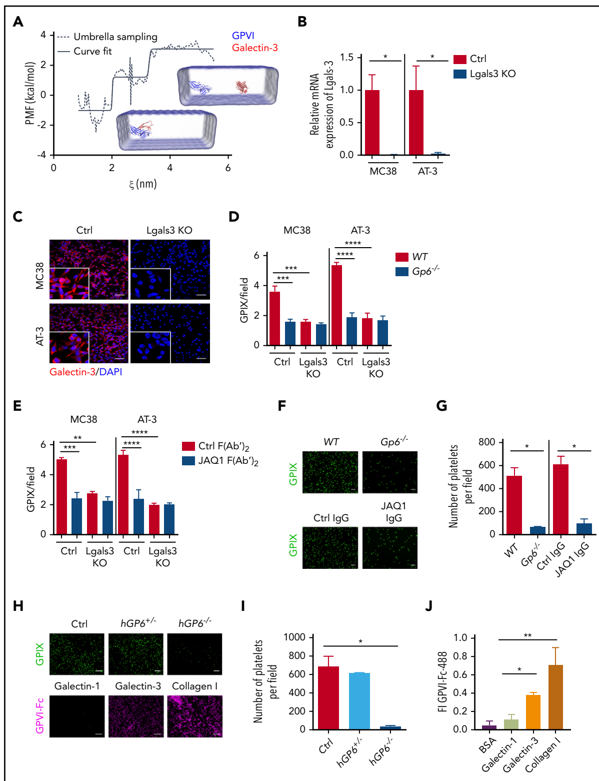
Figure 3. Galectin-3 expressed on tumor cells supports GPVI-dependent platelet adhesion. (A) Prediction of binding affinity between galectin-3 (red) and GPVI (blue). Graphs correspond to \Delta G_{\text{bind}} = -5.91 kcal/mol and K_D = 44.89 \mu\text{M} , respectively. Potential of mean force (PMF) values were extracted by the weighted histogram analysis method, which yields the binding free energy ( \Delta G_{\text{bind}} ) for the binding and unbinding processes. The \Delta G_{\text{bind}} value was calculated as the difference between the highest and lowest values of the PMF curve. The K_D of the protein-protein complex was calculated from the \Delta G_{\text{bind}} value according to the following equation: K_D = \exp(\Delta G_{\text{bind}}/R \cdot T) , where R (gas constant) is 1.98 cal/(mol·K) -1 and T (room temperature) is 298.15 Kelvins (K). The Boltzmann (sigmoidal) nonlinear fitting ( R^2 = 0.85 ; RMSE (root mean square error) = 0.67 ; RSS (residual sum of squares) = 88.31 ) of the data set is shown to assess the PMF elevation pattern with the increase of reaction coordinate ( \xi ), using the scaled Levenberg-Marquardt algorithm with tolerance = 0.0001 . (B-C) Knockout of the galectin-3 gene (Lgals3 KO) expression in MC38 and AT-3 cells. (B) Galectin-3 mRNA expression was determined by quantitative reverse transcription polymerase chain reaction and normalized with a messenger RNA level of glyceraldehyde-3-phosphate dehydrogenase. Data are presented as the mean \pm standard deviation (SD) of 4 separate cell culture experiments; * P < .05 , by Mann-Whitney test. (C) Representative immunofluorescence images of galectin-3
