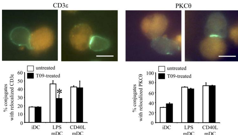
Figure 6. LPS- but not CD40L-matured LXR agonist-treated DCs fail to induce IS formation. Immature DCs (iDCs) were differentiated for 7 days and left untreated (control) or treated from day 2 on with 2 \mu M of the LXR agonist T0901317 (T09). Mature DCs were obtained from iDCs by incubation with LPS or CD40L for the last 2 days. Mature DCs were pulsed with superantigen for 30 minutes and incubated with Jurkat T cells for an additional 30 minutes. CD3 \epsilon and PKC \theta relocalization was visualized by indirect immunofluorescence. Typical examples of conjugates, negative (left) or positive (right) for relocalization of CD3 \epsilon and PKC \theta , are shown. Bar represents 10 \mu m. The diagram shows the percentage of conjugates counted positive for CD3 \epsilon and PKC \theta relocalization in means \pm SEM of 4 independent experiments. Significance versus untreated mDCs: * P \leq .05 .
