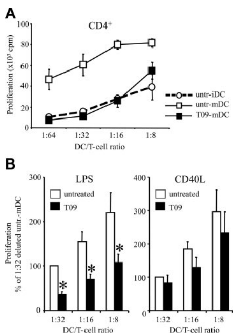
Figure 4. LPS- but not CD40L-matured LXR agonist-treated DCs fail to stimulate T cells. (A) Immature DCs (iDCs) were differentiated for 7 days and left untreated (control) or treated from day 2 on with 2 \mu M of the LXR agonist T0901317 (T09). Mature DCs were obtained from iDCs by incubation with LPS for the last 2 days. At day 7, immature and LPS-matured DCs were washed extensively, irradiated, and cocultured with 1 \times 10^5 allogeneic purified CD4 + T cells at the indicated ratios. After 4 days, proliferation was measured by [ 3 H]-thymidine incorporation in 4 independent experiments. (B) Allogeneic MLRs were performed as described for panel A using LPS- and CD40L-matured DCs, respectively. * P \leq .05 for difference between T09-treated versus untreated DCs. Data show the means and SEM of 4 independent experiments.
